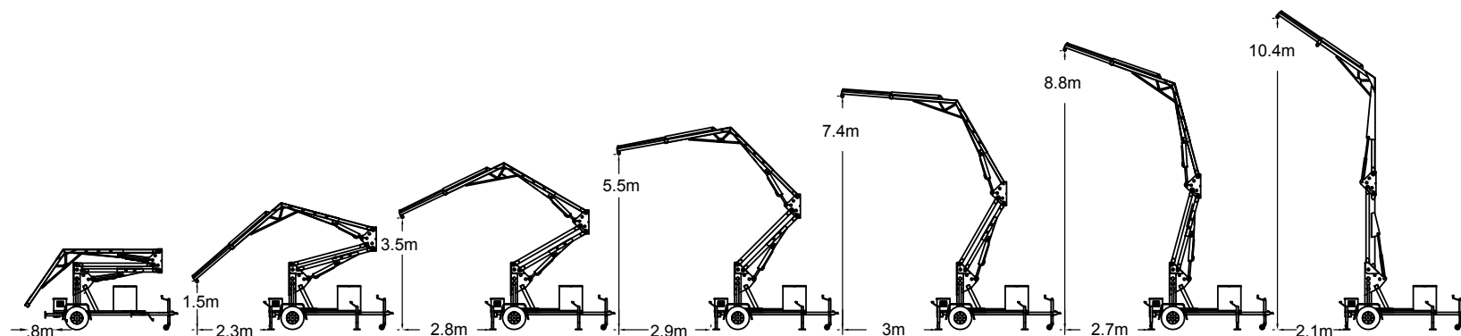
X1250 Mobile Grabber Reach Chart
